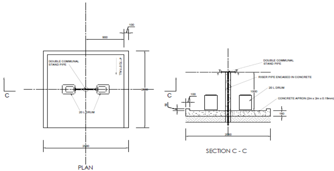
DOUBLE COMMUNAL TAP DETAIL
